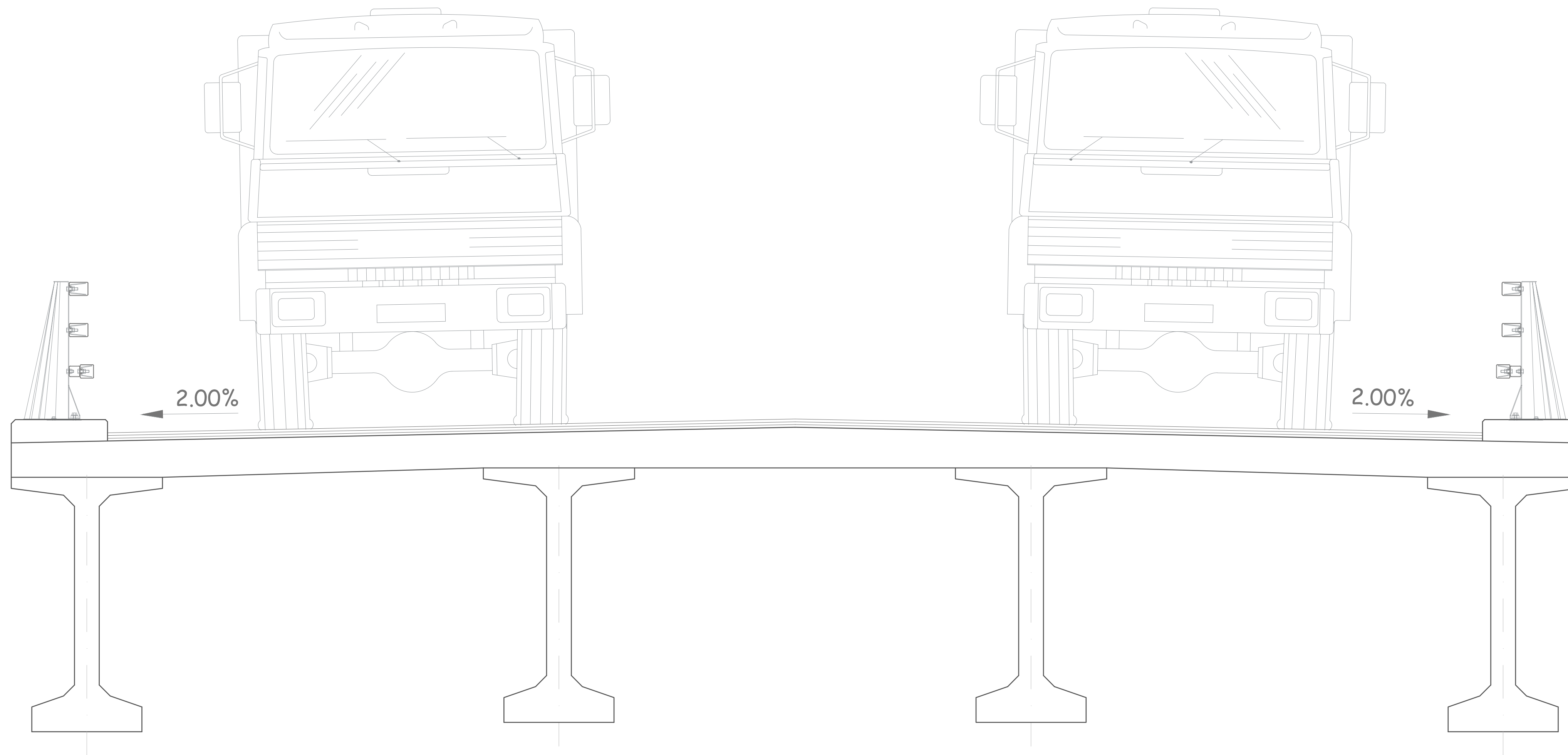
Front Elevation
