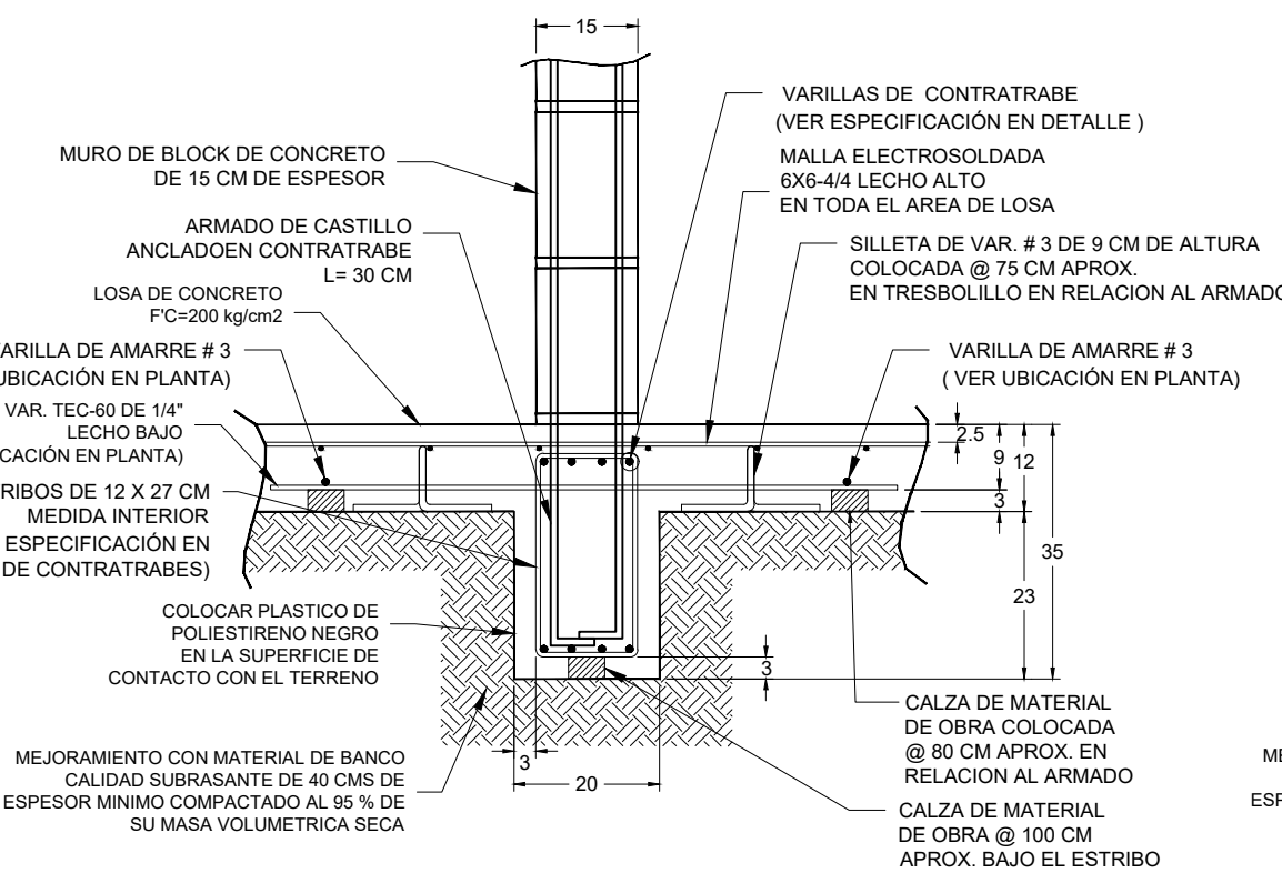
DETALLE 3-3' DE CONTRATRABE INTERIOR
