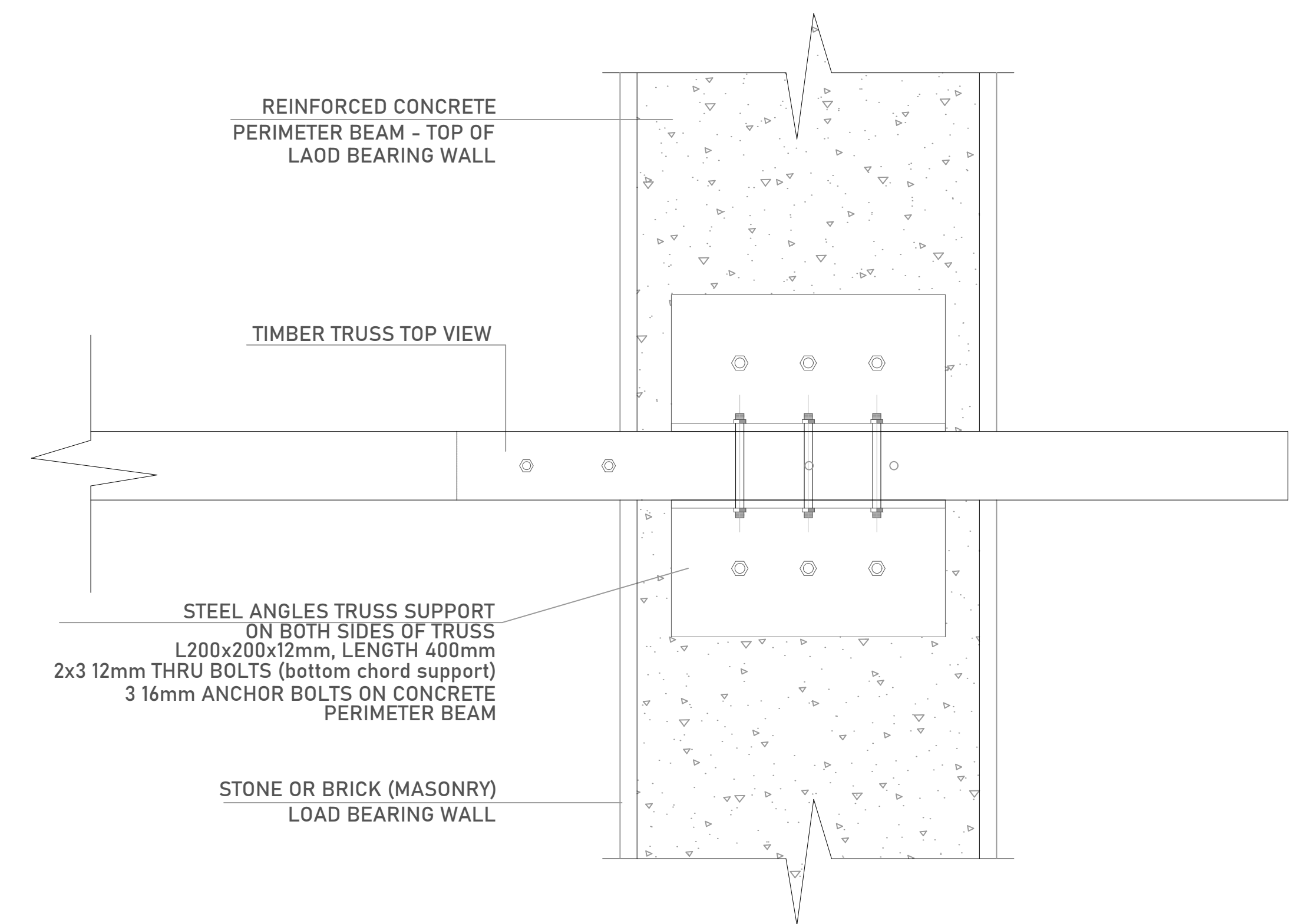
TOP VIEW
