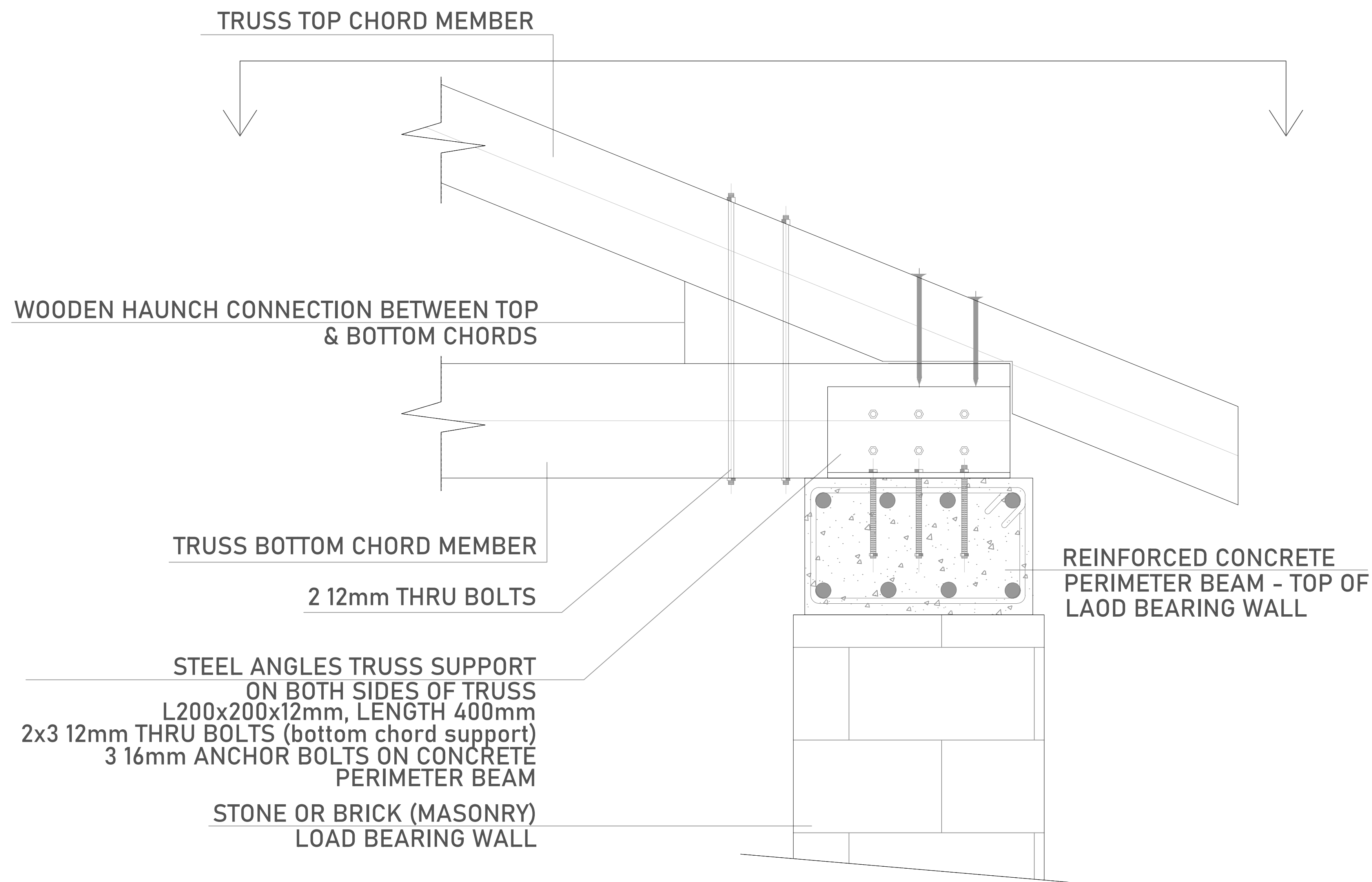
ELEVATION VIEW
